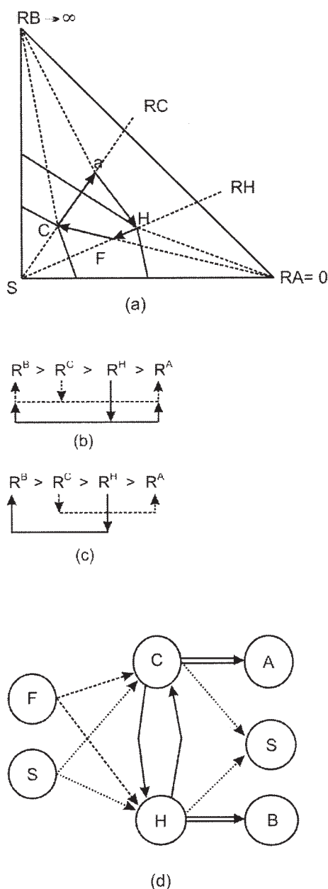
Figure 2. Design of a separation sequence for a simple system.
