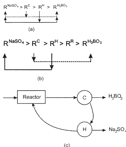
Figure 12. Production of boric acid starting with ulexite.
