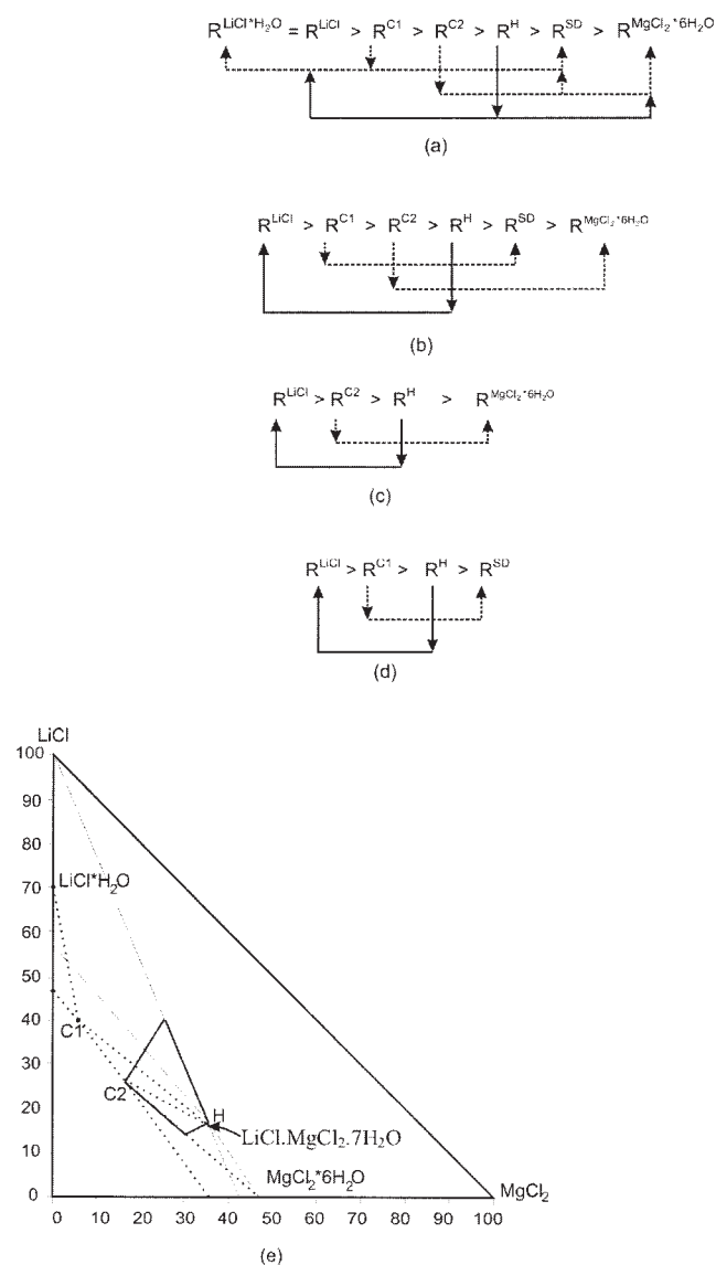
Figure 5. Lithium chloride and magnesium chloride system.
