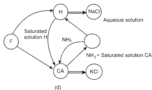
Figure 13. Separation of sylvinites using ammonia as a drowning-out agent.
