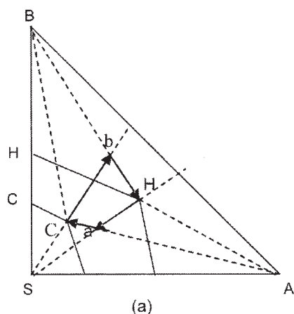
Figure 1. Isothermal sections and a partial separation cycle.
