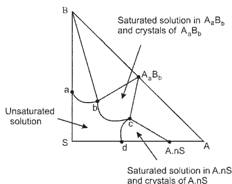
Figure 3. Phase diagram for a system with compound formation.
