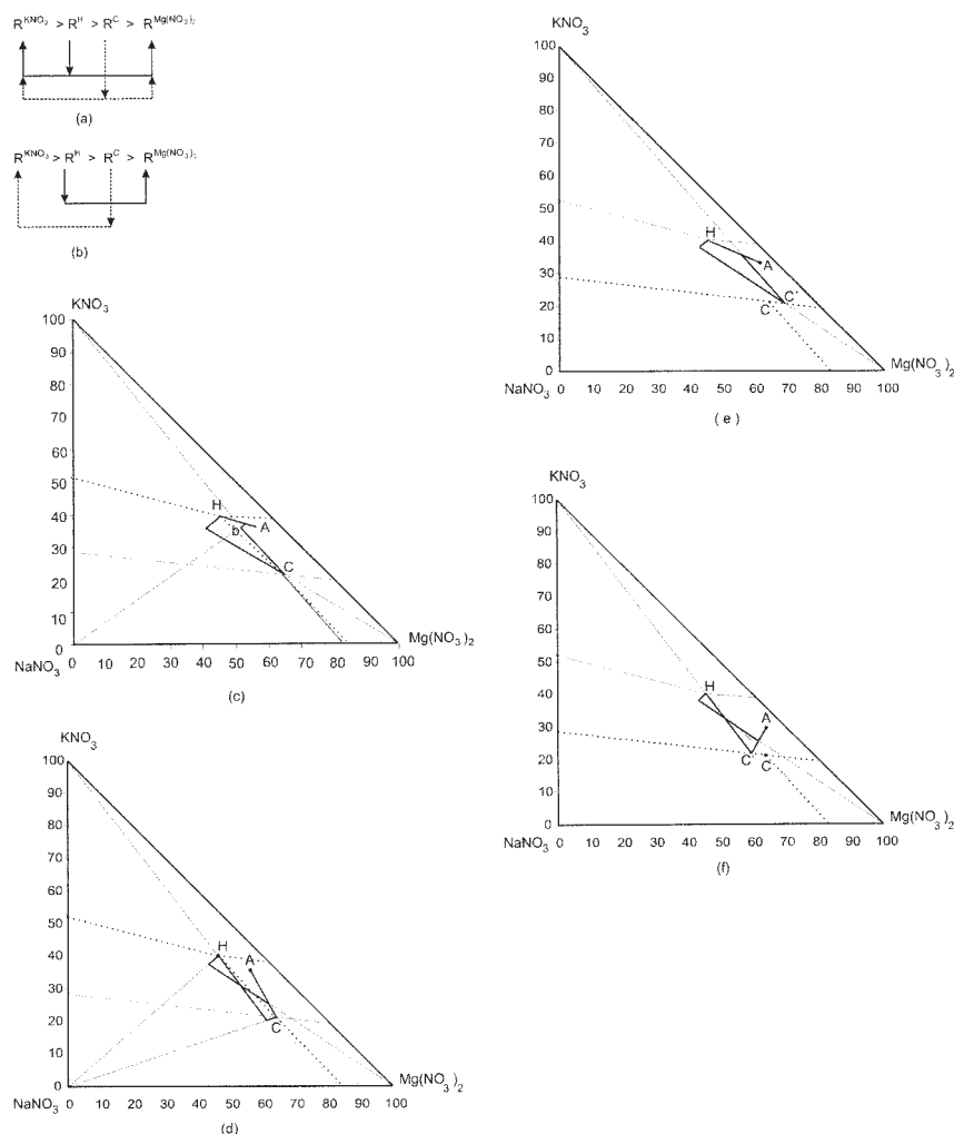
Figure 10. \text{KNO}_3 + \text{Mg}(\text{NO}_3)_2 + \text{NaNO}_3 + \text{water} system.
