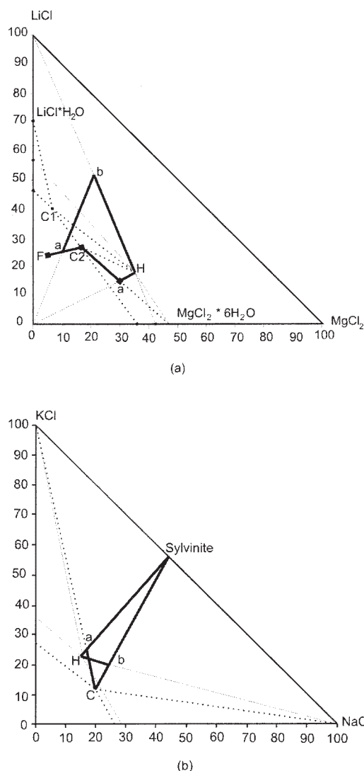
Figure 8. (a) Management of feed in the example in Figure 7b for the lithium chloride and magnesium chloride system; (b) management of the feed in the separation of sylvinite.
